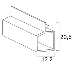
TERPVCPLA in PVC super 13,2x20,5 mm
