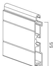
T55 in alluminio 14x55 mm
