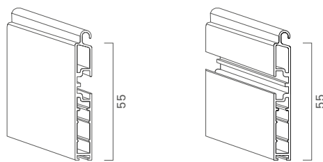
T45 in alluminio 9x55 mm
