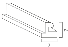
TERPVC45 in gomma 17x7 mm
