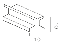
TERPVCDO in gomma 10x10 mm
